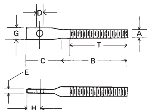
Spade Bolt
