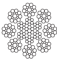
8x19 (9/9/1) AA SEALE
