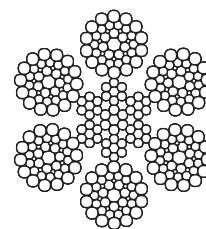
6x43 (14/14/7/7/1) AA FILLER SEALE
