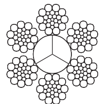
6x26 (10/5+5/5/1) AF WARRINGTON SEALE
