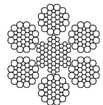
6x31 (12/6+6/6/1) AA WARRINGTON SEALE
