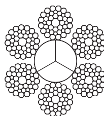
6x41 (16/8+8/8/1) AF WARRINGTON SEALE
