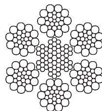
6x26 (10/5+5/5/1) AA WARRINGTON SEALE
