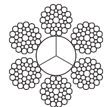
6x36 (14/7+7/7/1) AF WARRINGTON SEALE
