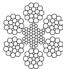
6x21 (10/5/5/1) AA FILLER
