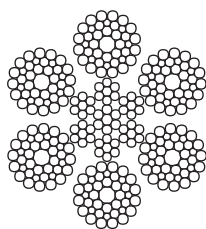
6x41 (16/8+8/8/1) AA WARRINGTON SEALE
