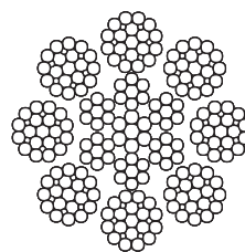
8x25 (12/6/6/1) AA FILLER
